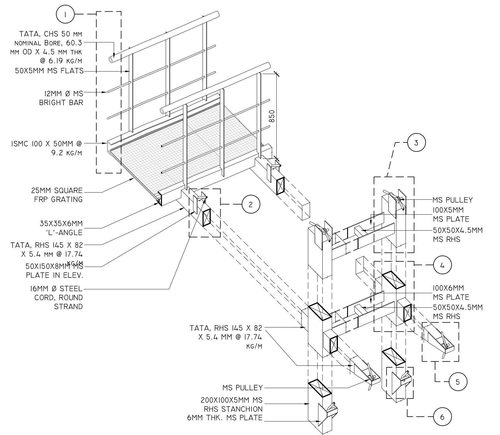
CATWALK ISOMETRIC DETAIL
