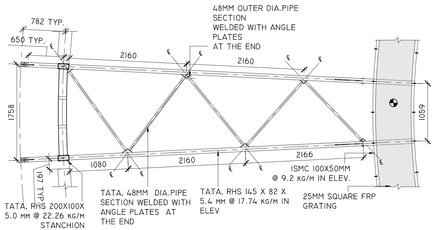
PART PLAN
