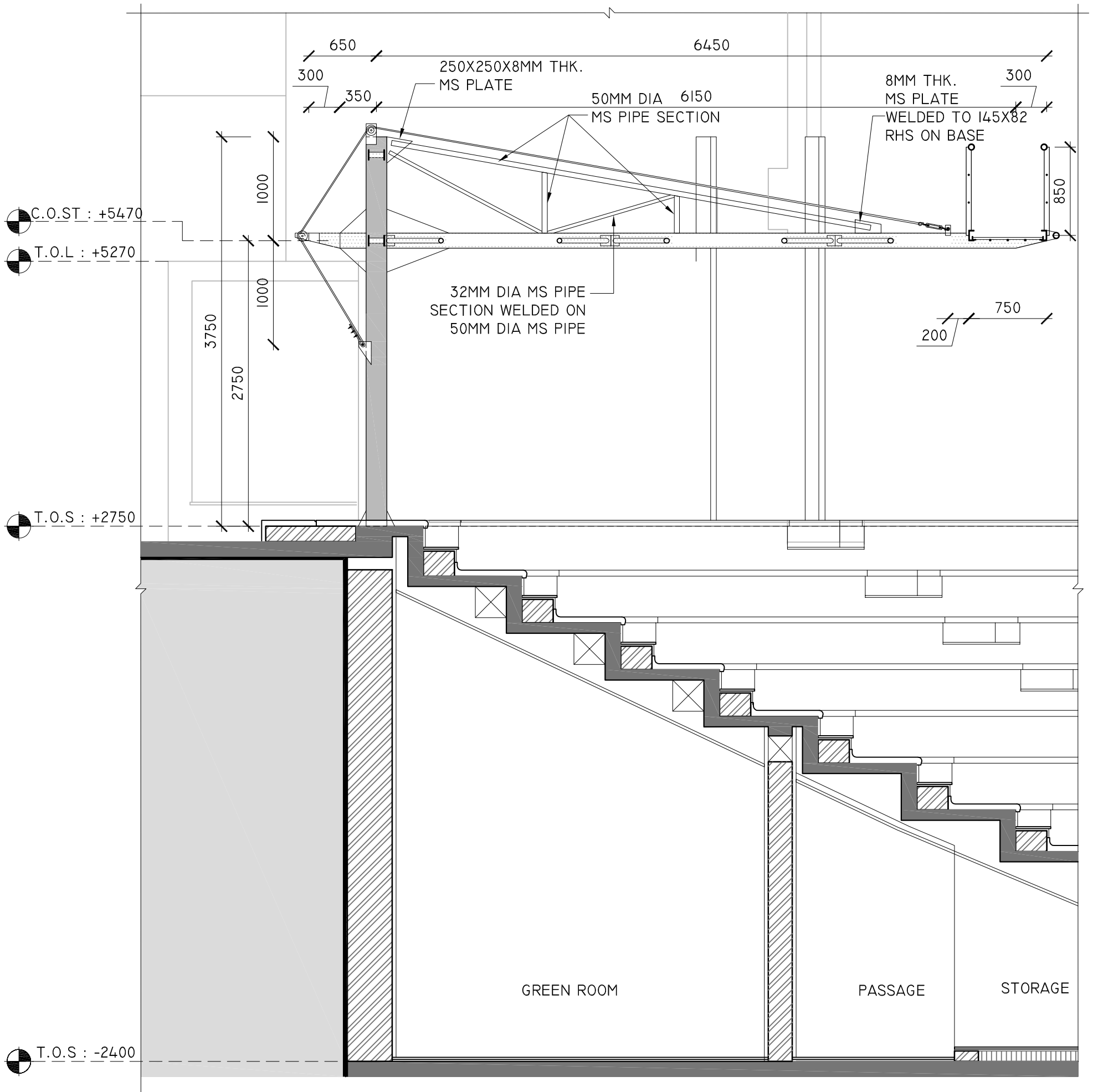
SECTION
