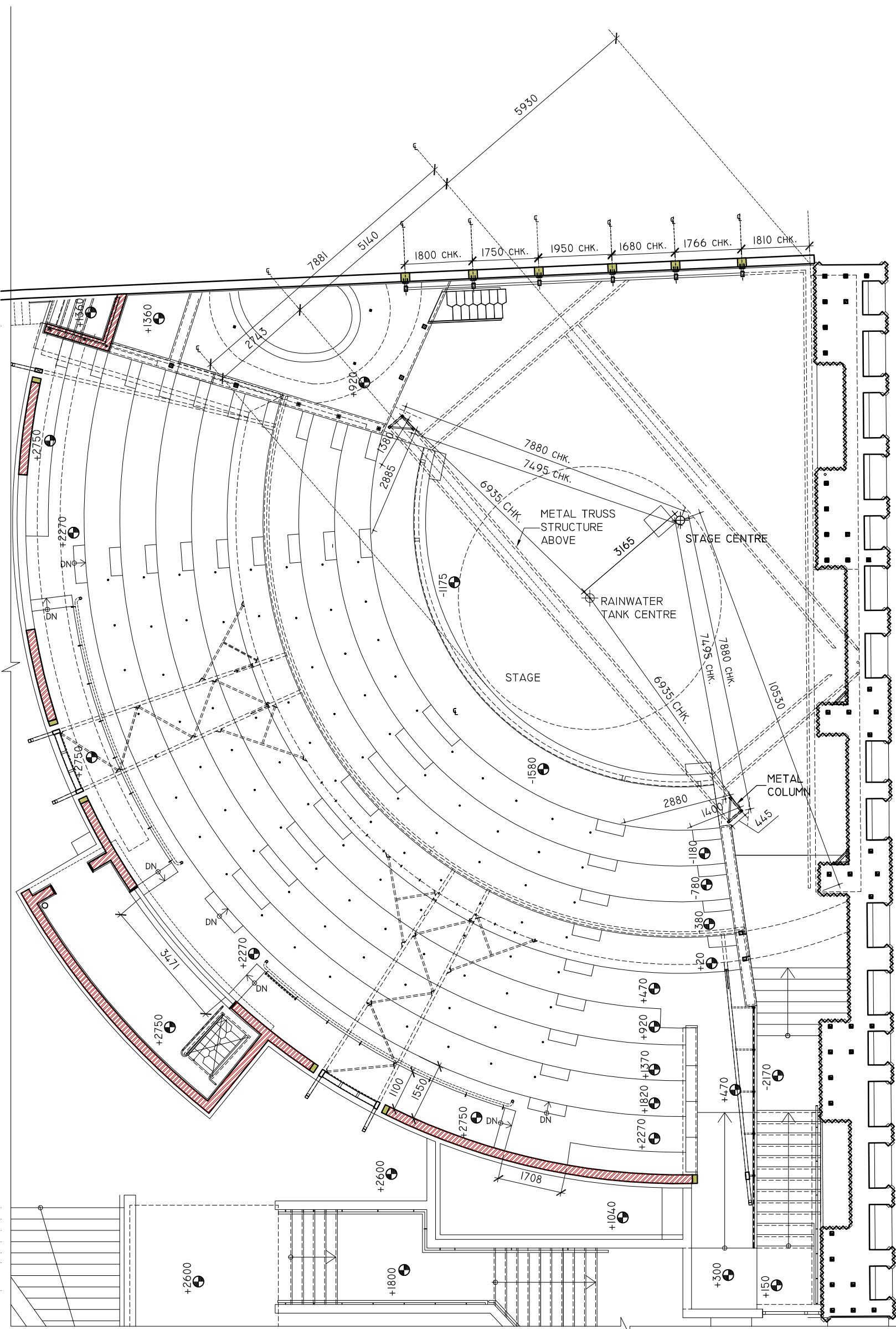
PLAN AT +3700MM.
