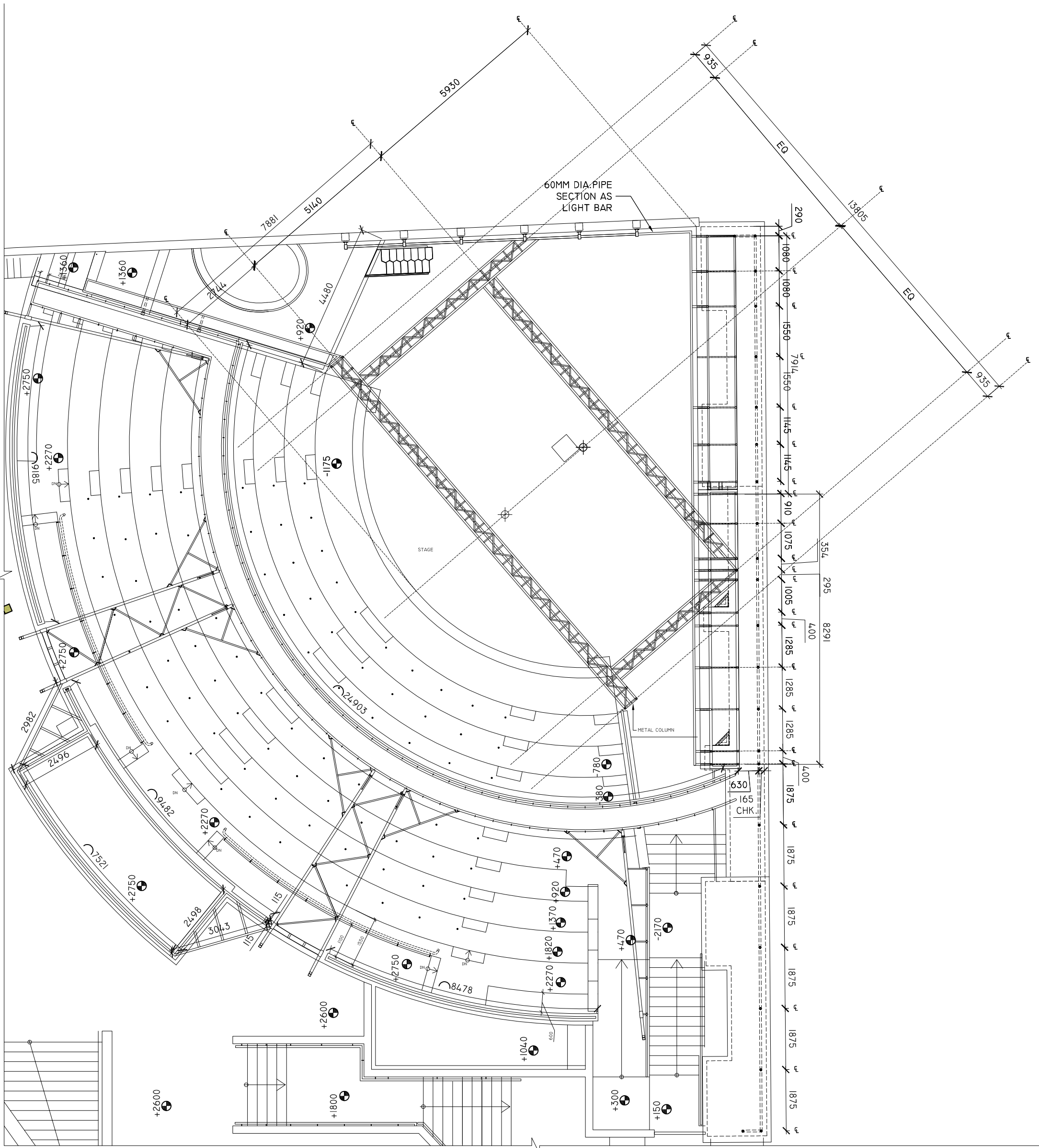
PLAN AT +7600MM.
