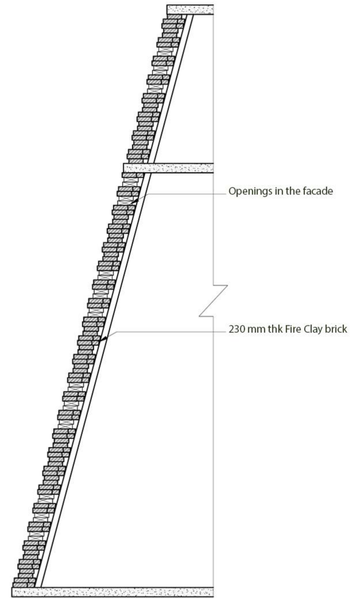
SECTION S1 FOR THE JALI DETAIL (SCALE 1:100)
