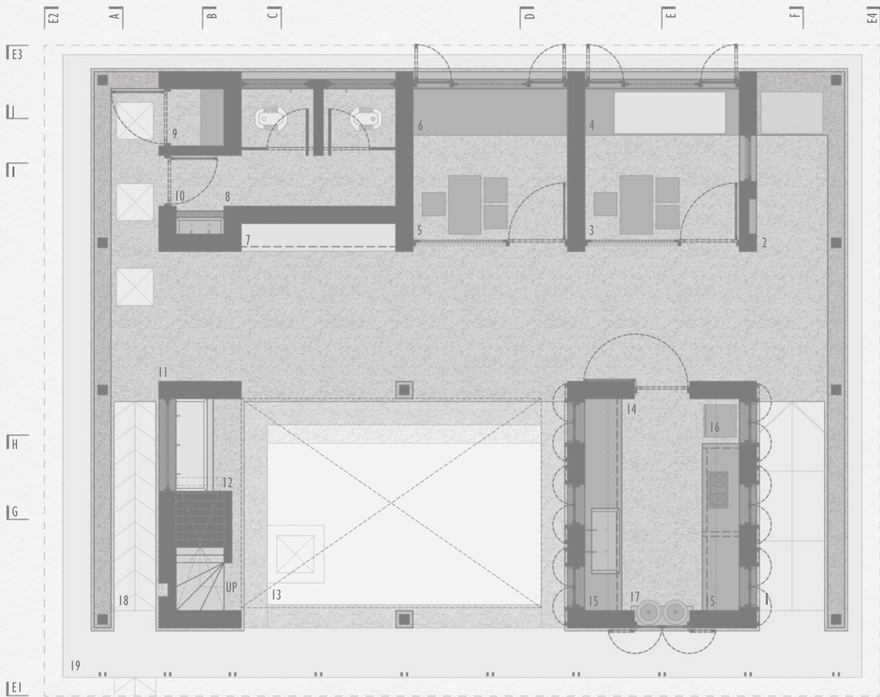
1-Main entrance 2-Waiting area-clinic 3-Clinic 4-Examination table 5-Office 6-Work station 7-Common storage 8-Toilet 9-MDB room 10-Handwash 11-Multifunctional space 12-Common wash 13-O.T.S courtyard 14-Kitchen 15-Cooking platform 16-Fridge 17-Drinking water pots 18-Secondary entrance 19-Verandah
